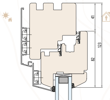
SECTION VERTICALE A-A
