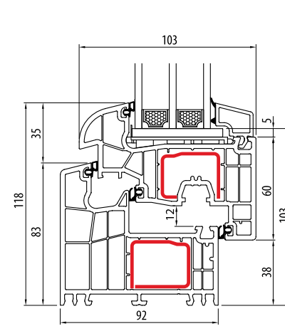
Bluevolution 92 Round-line
