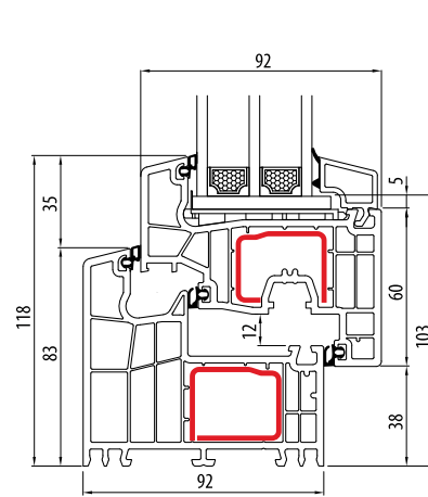
Bluevolution 92 Classic-line
