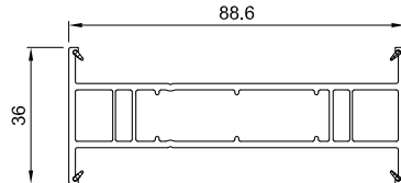
NP8170
